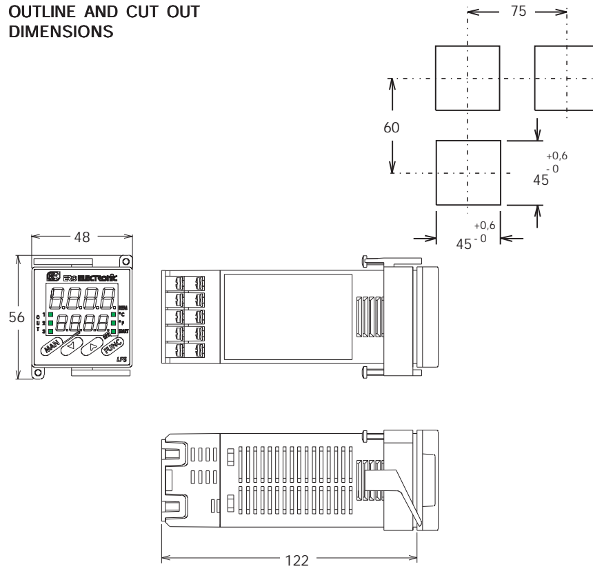
Fig. 2 OUTLINE AND CUT-OUT DIMENSIONS
