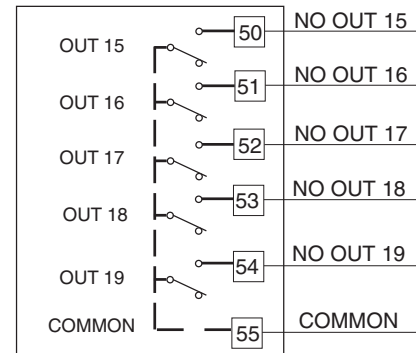
Fig. 11.C RELAY OUTPUTS 15 to 19 WIRING
