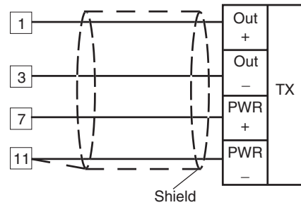
Fig. 7.C INPUTS WIRING FOR 4-WIRE TRANSMITTER
