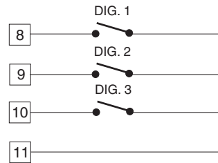
Fig. 9.A - LOGIC INPUTS DIG.1, 2 and 3 WIRING
