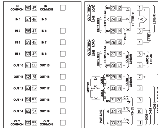
Fig. 3.B MKC REAR TERMINAL BLOCK
