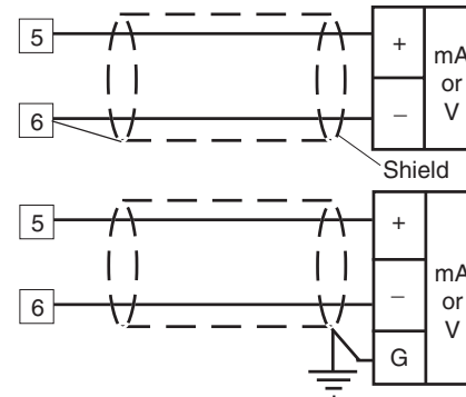
Fig. 8 AUXILIARY INPUT WIRING
