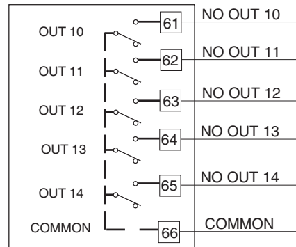
Fig. 11.B RELAY OUTPUTS 10 to 14 WIRING
