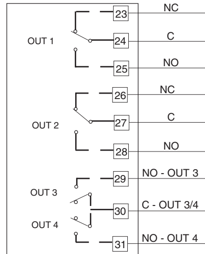
Fig. 11.A RELAY OUTPUTS 1,2,3 and 4 WIRING
