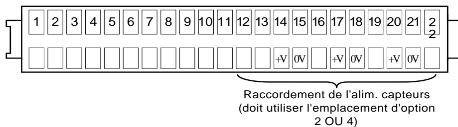
Figure 10.2 Brochage TRS
