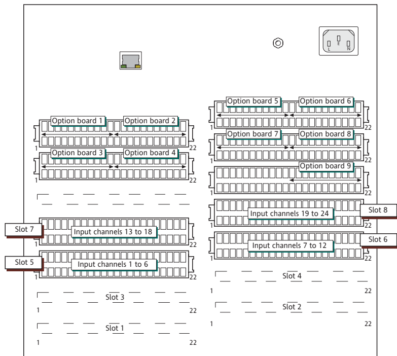
Figure 1 Connector locations (6180A shown - 5180V similar)
